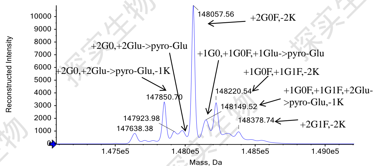
● Reconstruction from Training_MW_W_20220302.w...xperiment 1 @ RT: 5.92 from 5.88 to 5.98 min
