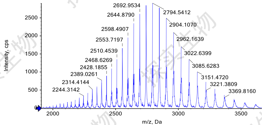
● +TOF MS from Training_MW_W_20220302.wiff2 (...xperiment 1 @ RT: 5.92 from 5.88 to 5.98 min
